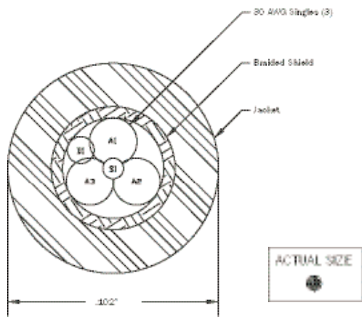
3 Conductor Cable: 3 - 30 AWG alloy singles cabled around core with drain wire, shielded and jacketed with PVC to 0.102" O.D.
