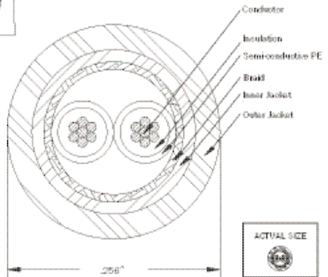
Audio Interconnect: 2 solid and stranded copper conductors insulated with Polyethylene, semi-conductive Polyethylene, braided and jacketed with two outside layers of PVC insulation to 0.256" O.D.
